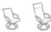
JJ360/JJ900 Std-Bk/Hi-Bk S/Rocker W:25" H:34.75/42.75" SH:17" D:30.75" W:63cm H:88/109cm SH:43cm D:78cm
